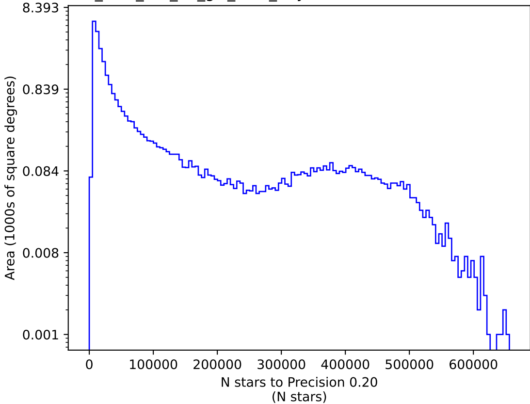
too_elab_r16_d3_giz_v3.4_10yrs i: N stars to Precision 0.20
