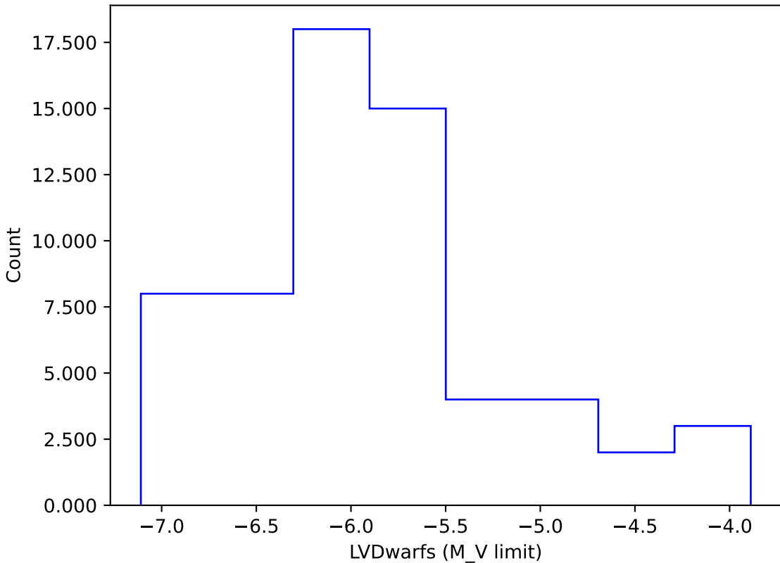
too_elab_r16_d3_giz_v3.4_10yrs gi: LVDwarfs
