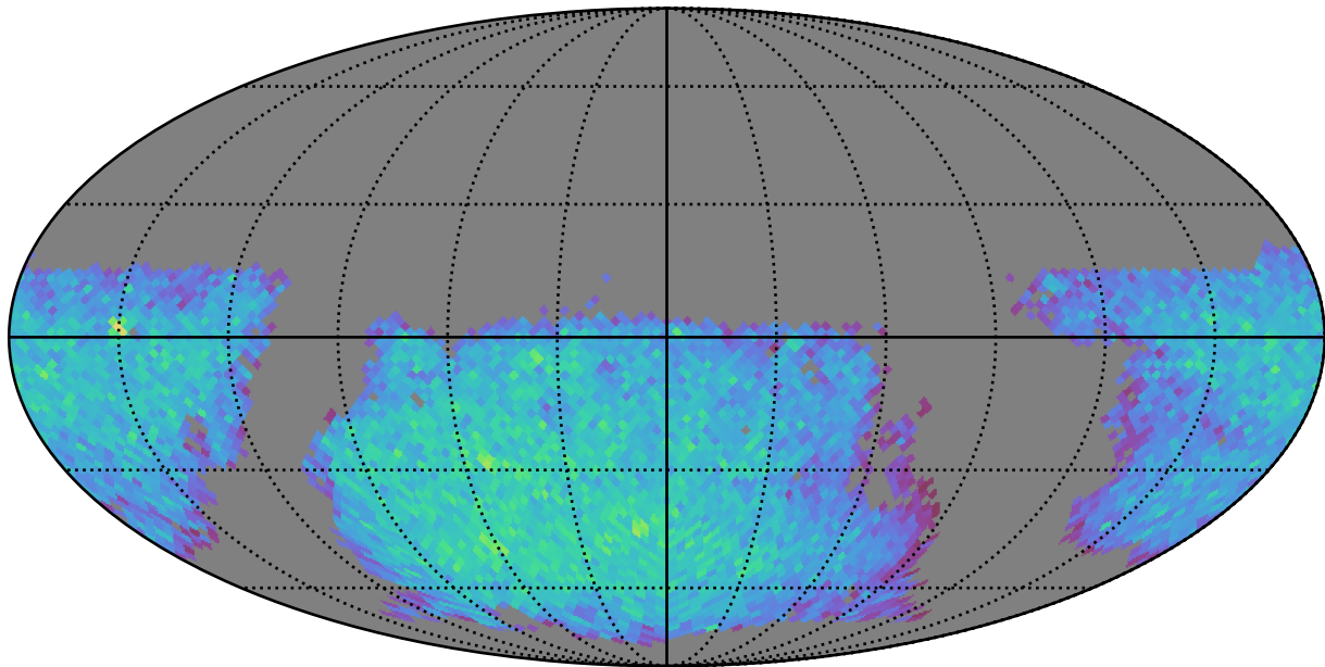
too_elab_r16_d3_giz_v3.4_10yrs gi: LVDwarfs
