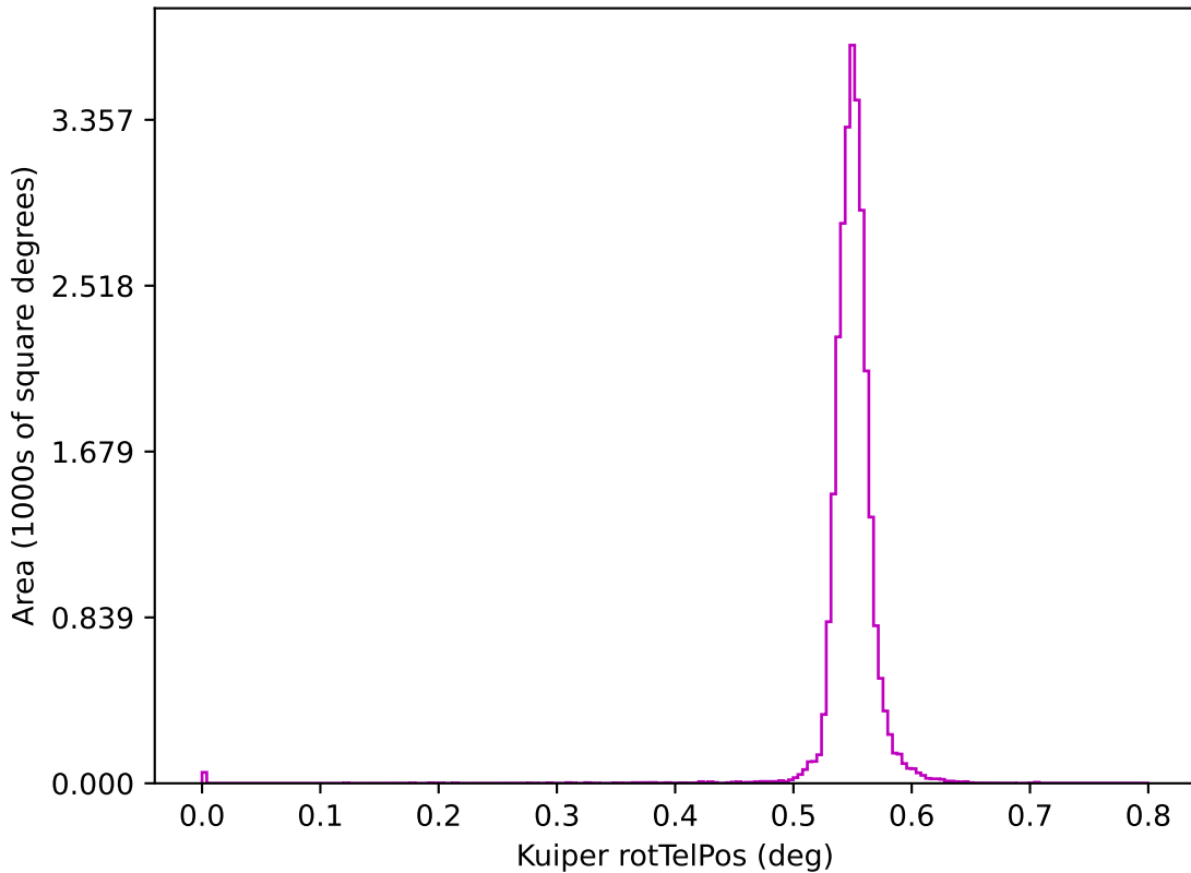
too_elab_r16_d3_giz_v3.4_10yrs z: Kuiper rotTelPos
