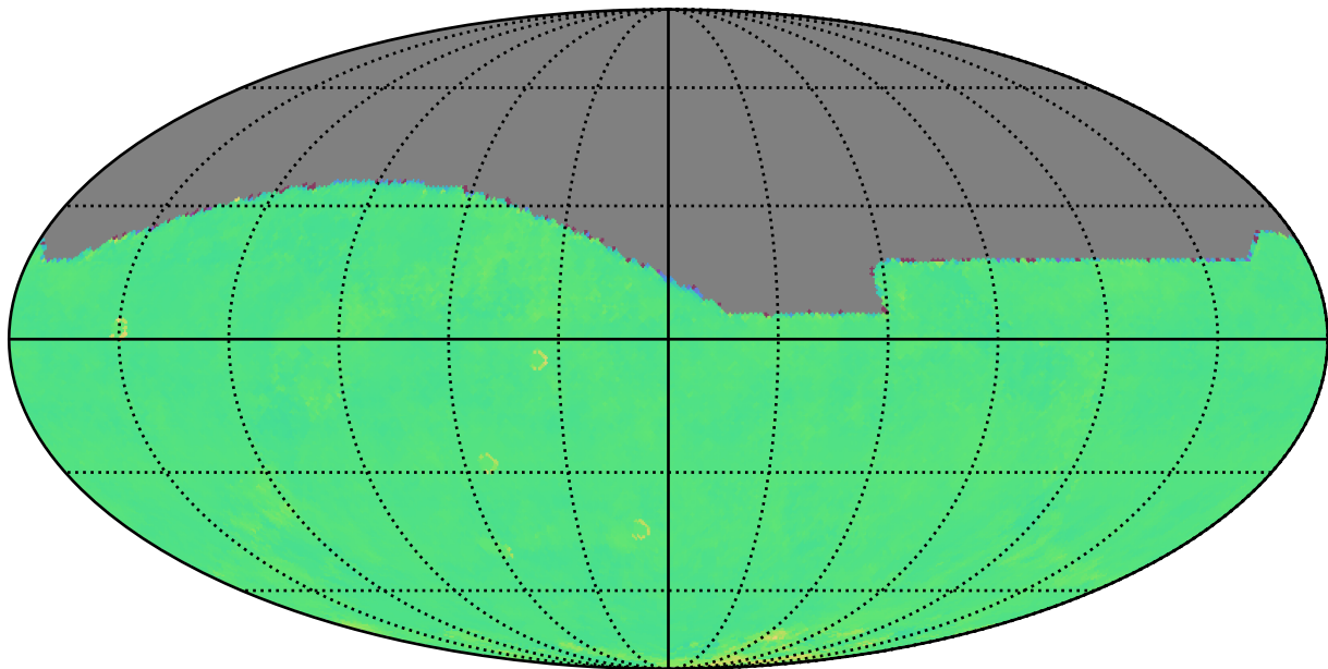
too_elab_r16_d3_giz_v3.4_10yrs r: Kuiper rotTelPos
