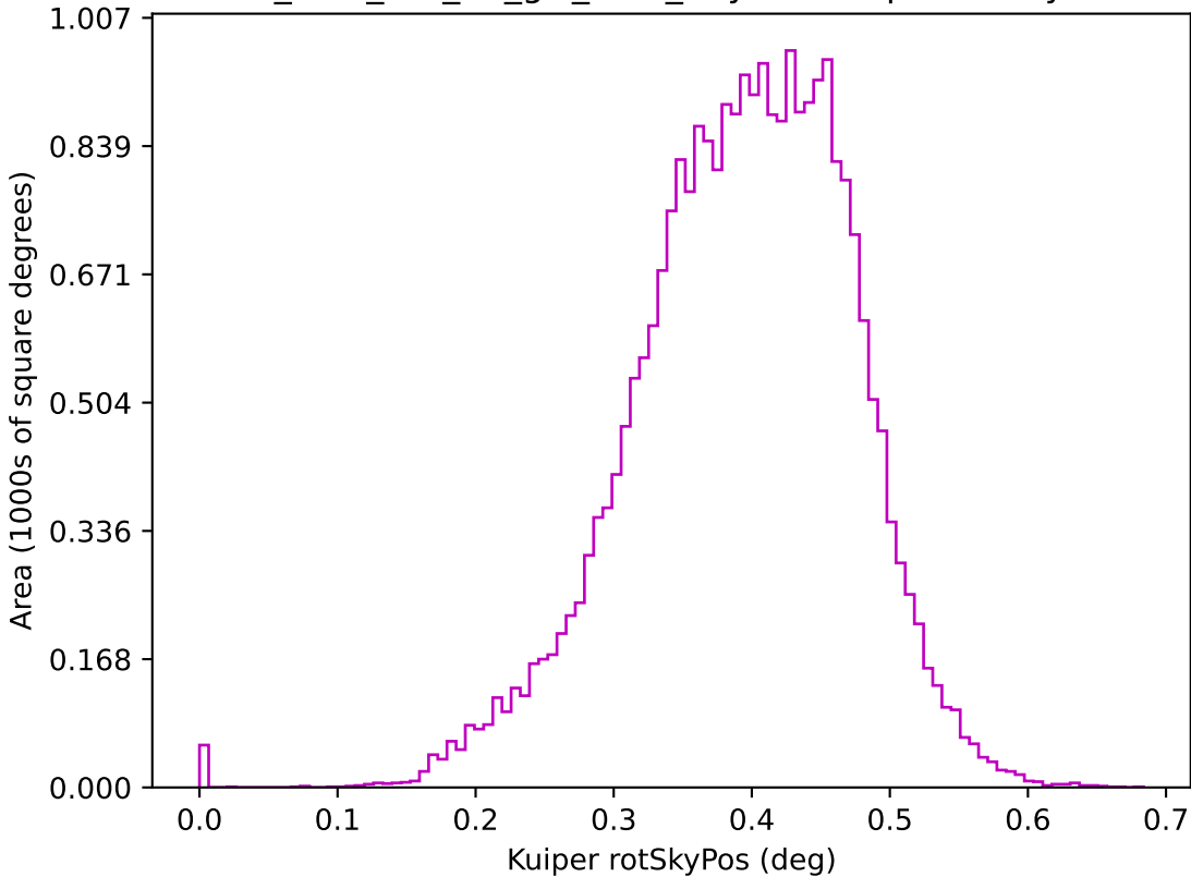
too_elab_r16_d3_giz_v3.4_10yrs z: Kuiper rotSkyPos
