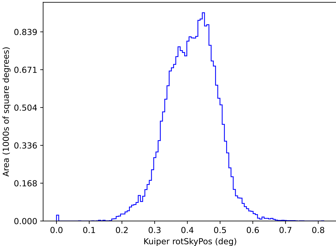
too_elab_r16_d3_giz_v3.4_10yrs y: Kuiper rotSkyPos
