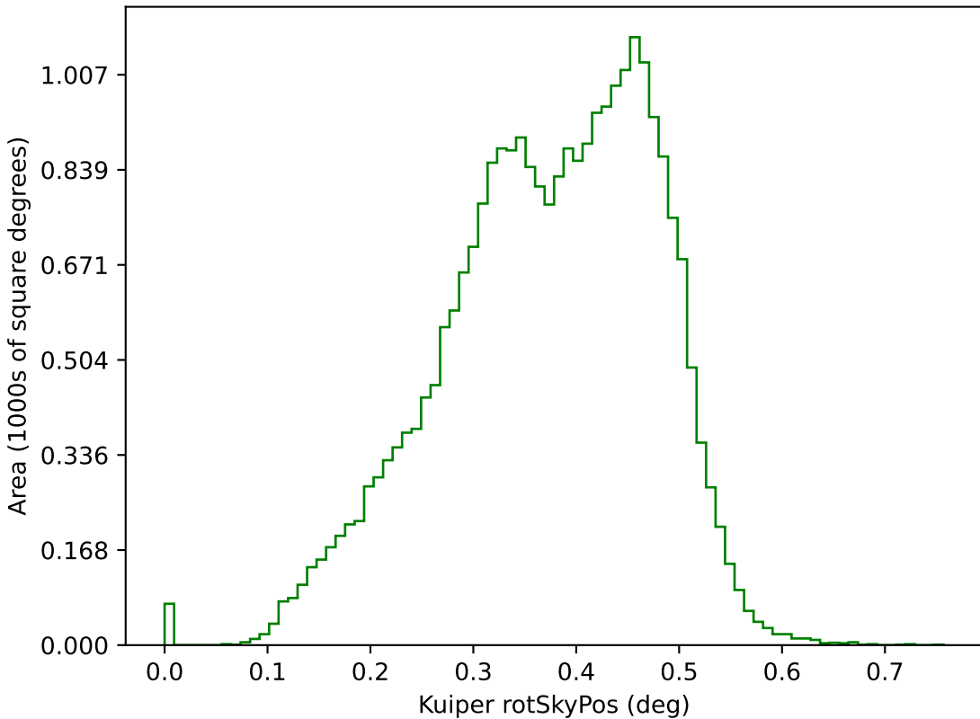
too_elab_r16_d3_giz_v3.4_10yrs g: Kuiper rotSkyPos
