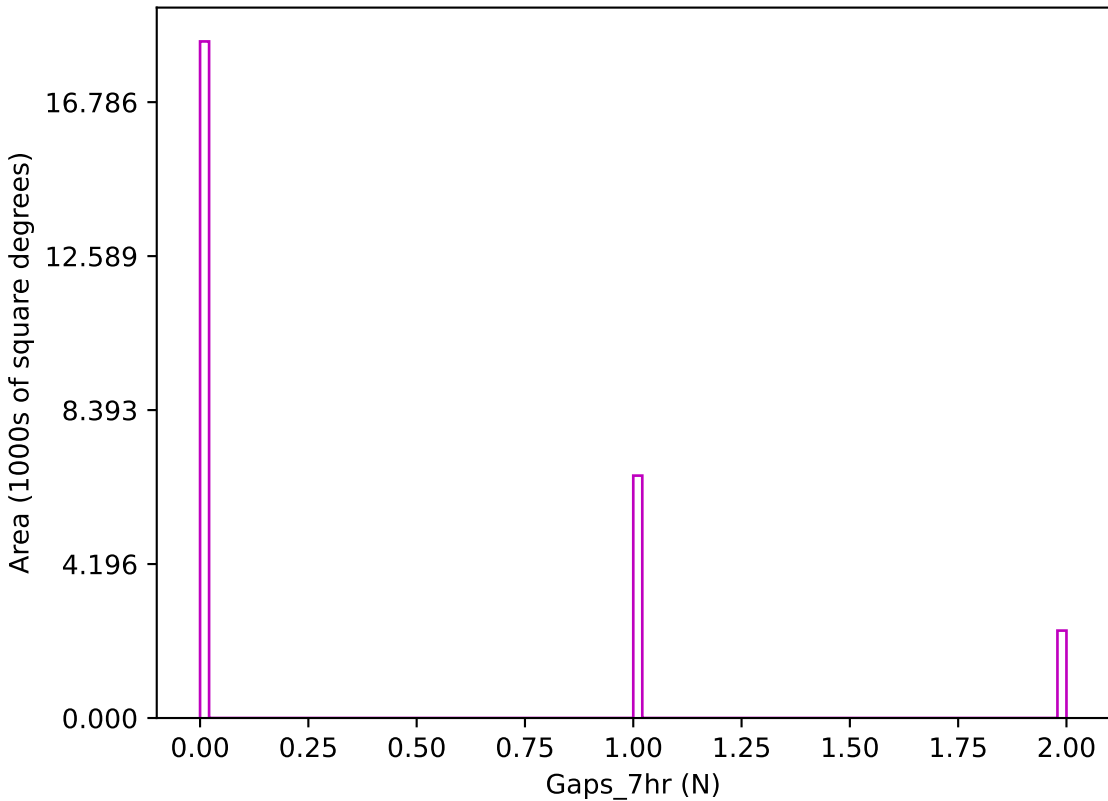
too_elab_r16_d3_giz_v3.4_10yrs z band: Gaps_7hr
