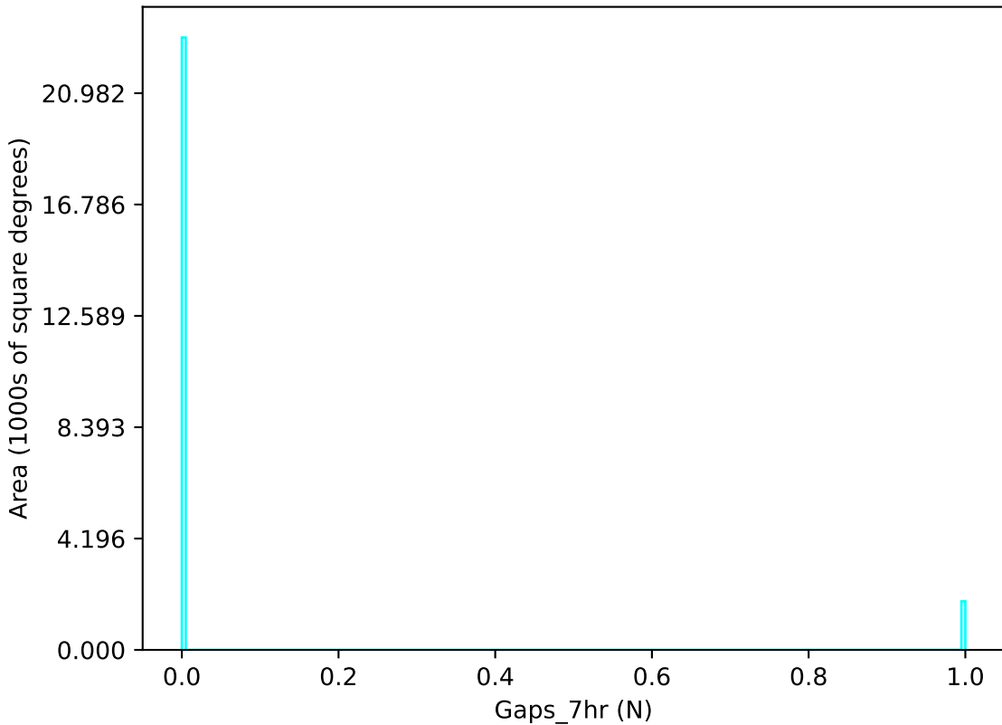
too_elab_r16_d3_giz_v3.4_10yrs u band: Gaps_7hr
