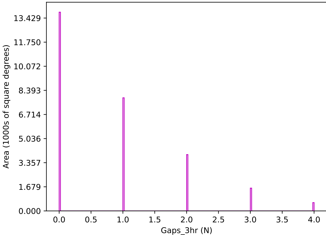
too_elab_r16_d3_giz_v3.4_10yrs z band: Gaps_3hr
