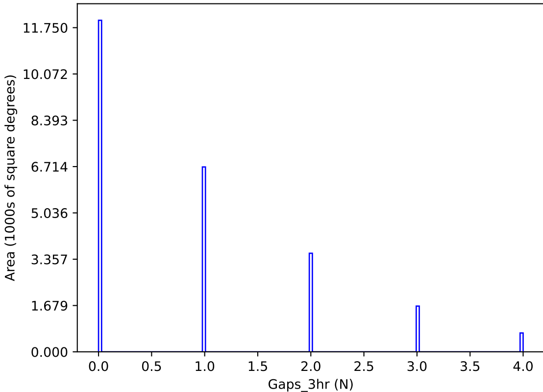
too_elab_r16_d3_giz_v3.4_10yrs y band: Gaps_3hr
