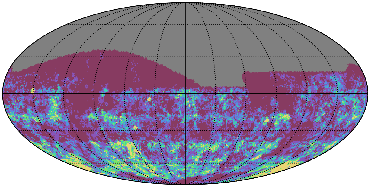
too_elab_r16_d3_giz_v3.4_10yrs r band: Gaps_3hr
