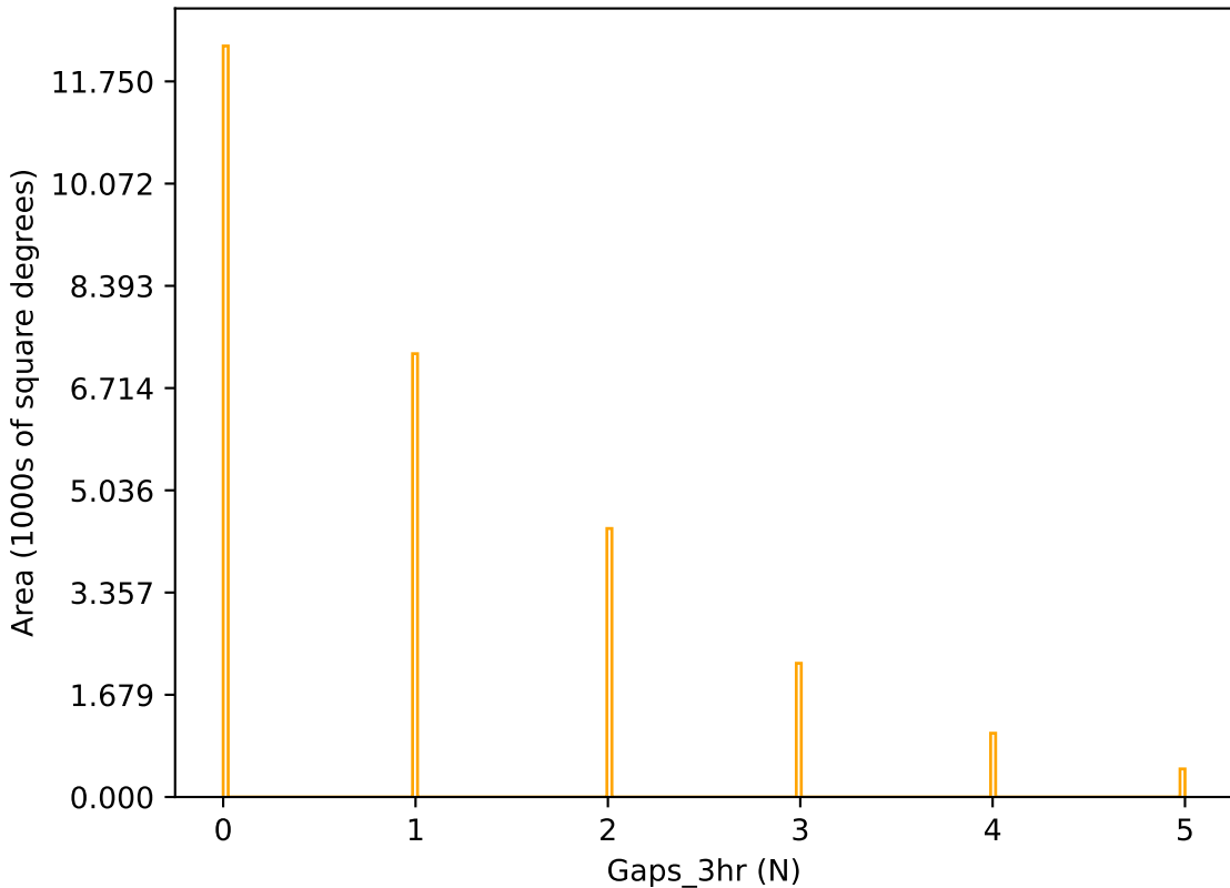
too_elab_r16_d3_giz_v3.4_10yrs r band: Gaps_3hr
