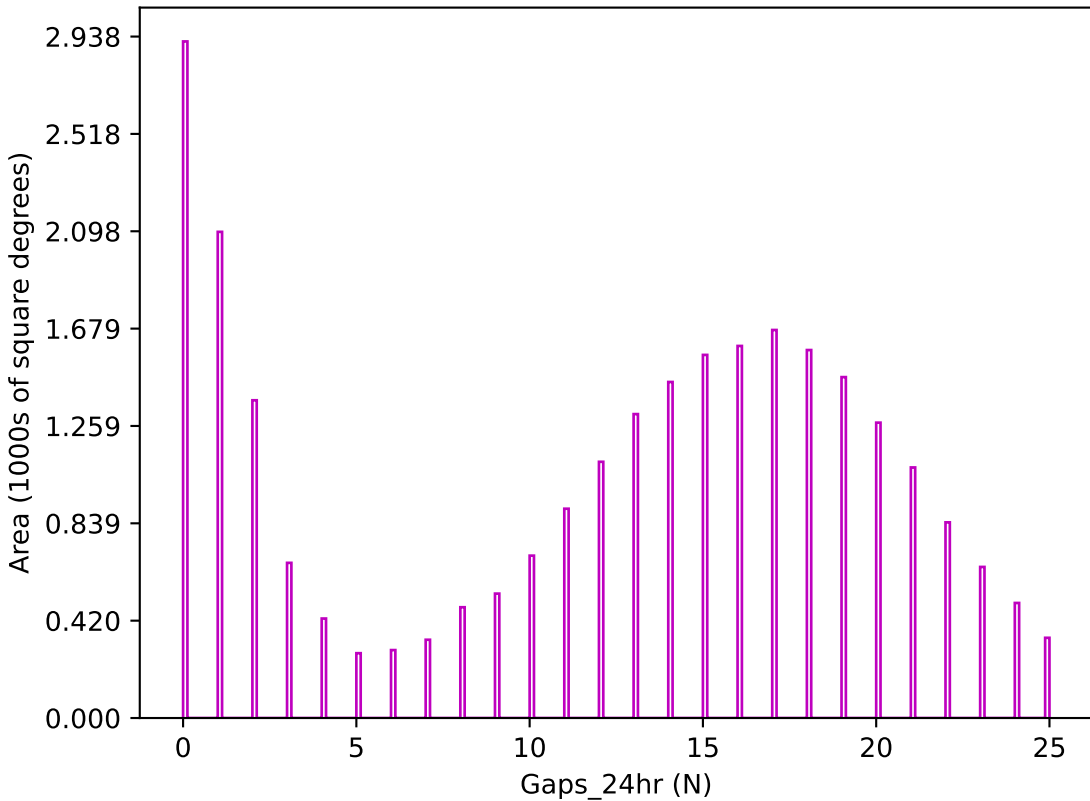
too_elab_r16_d3_giz_v3.4_10yrs z band: Gaps_24hr
