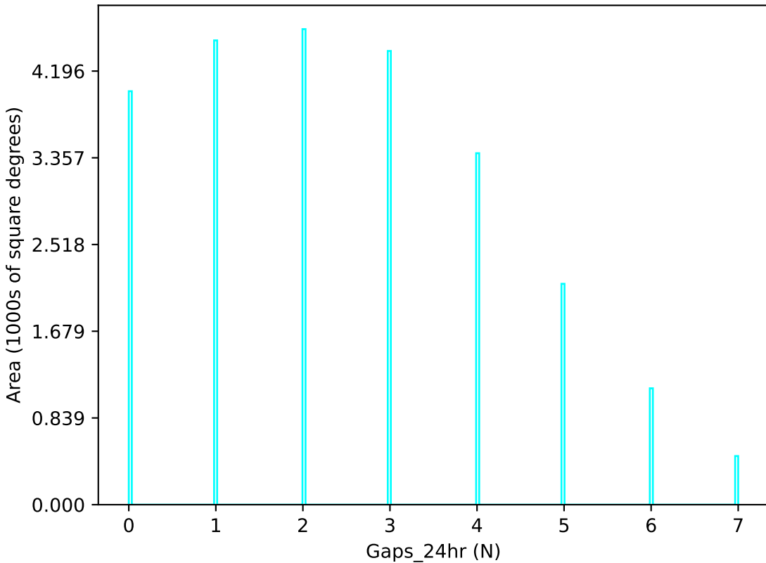
too_elab_r16_d3_giz_v3.4_10yrs u band: Gaps_24hr
