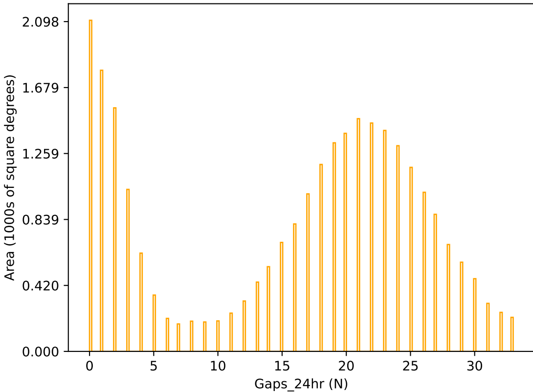
too_elab_r16_d3_giz_v3.4_10yrs r band: Gaps_24hr
