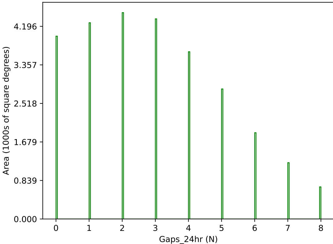
too_elab_r16_d3_giz_v3.4_10yrs g band: Gaps_24hr
