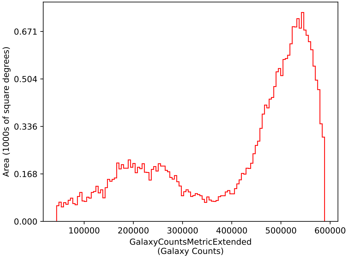
too_elab_r16_d3_giz_v3.4_10yrs i: GalaxyCountsMetricExtended
