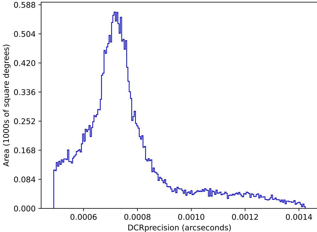
too_elab_r16_d3_giz_v3.4_10yrs : DCRprecision
