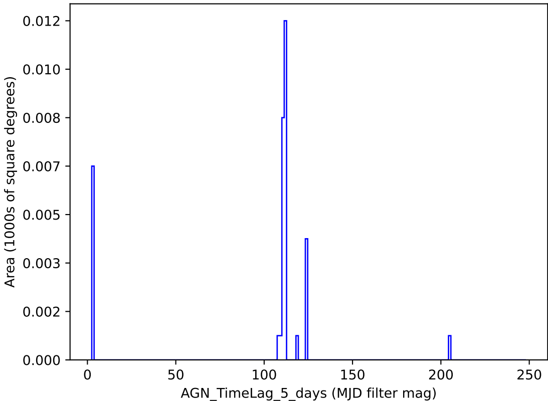
too_elab_r16_d3_giz_v3.4_10yrs y band: AGN_TimeLag_5_days
