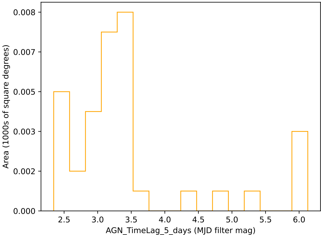
too_elab_r16_d3_giz_v3.4_10yrs r band: AGN_TimeLag_5_days
