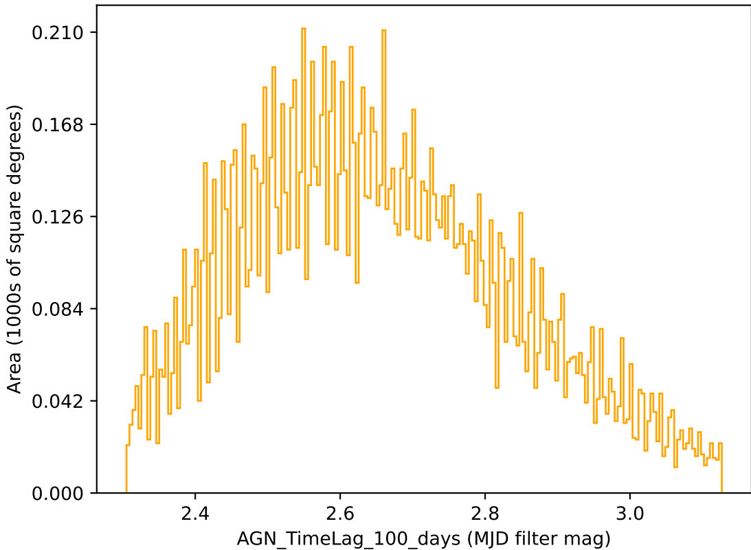
too_elab_r16_d3_giz_v3.4_10yrs r band: AGN_TimeLag_100_days
