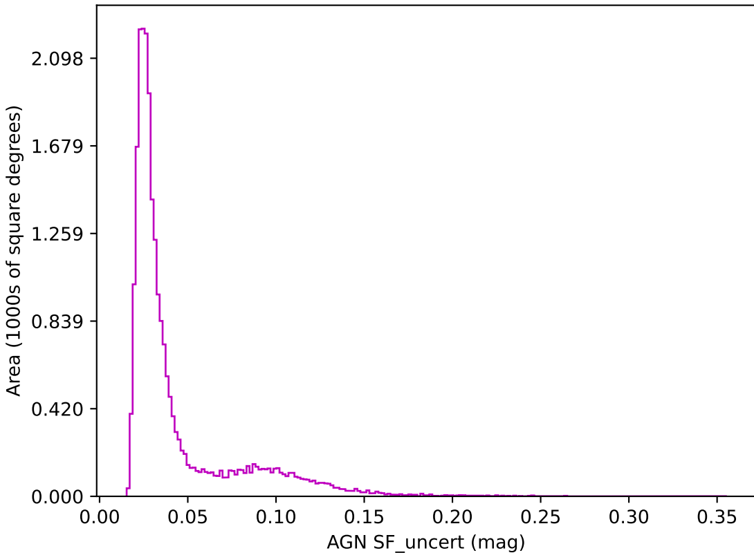
too_elab_r16_d3_giz_v3.4_10yrs z band: AGN SF_uncert
