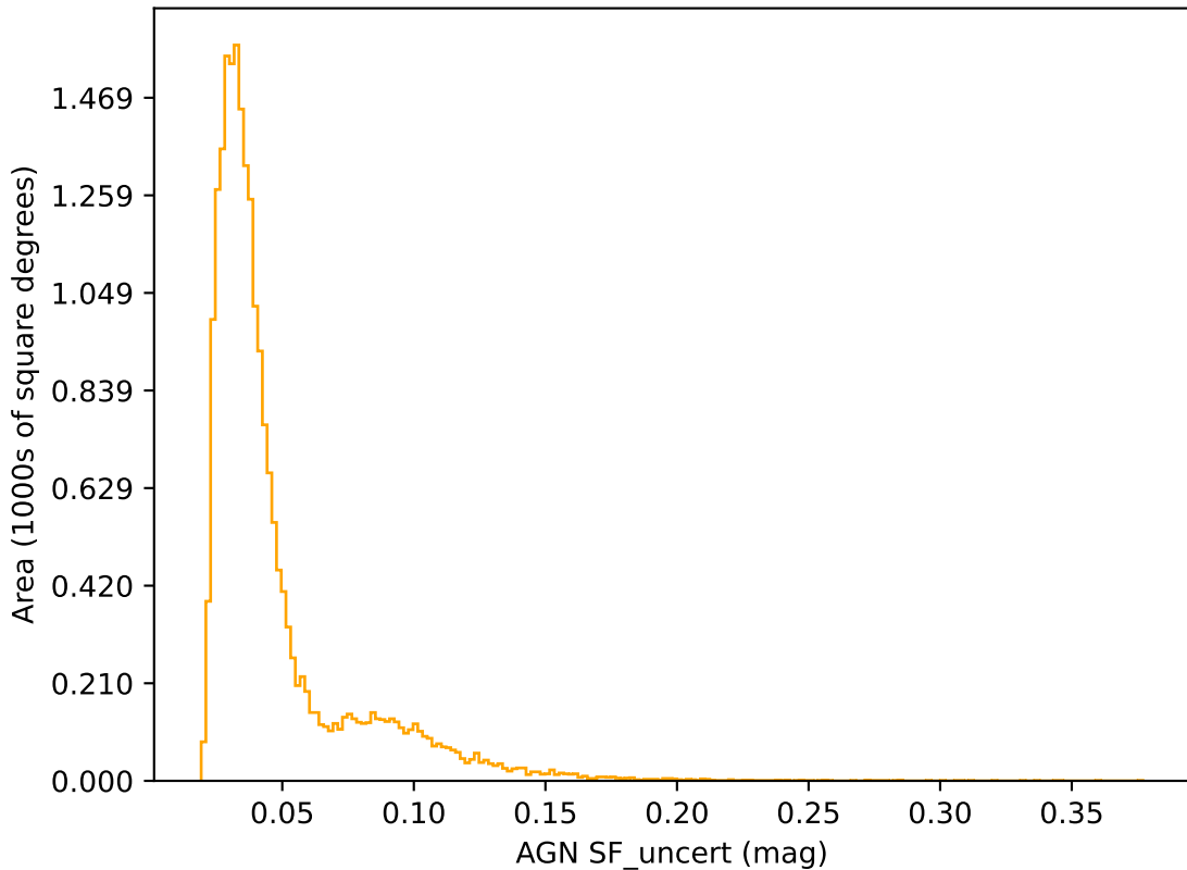
too_elab_r16_d3_giz_v3.4_10yrs r band: AGN SF_uncert
