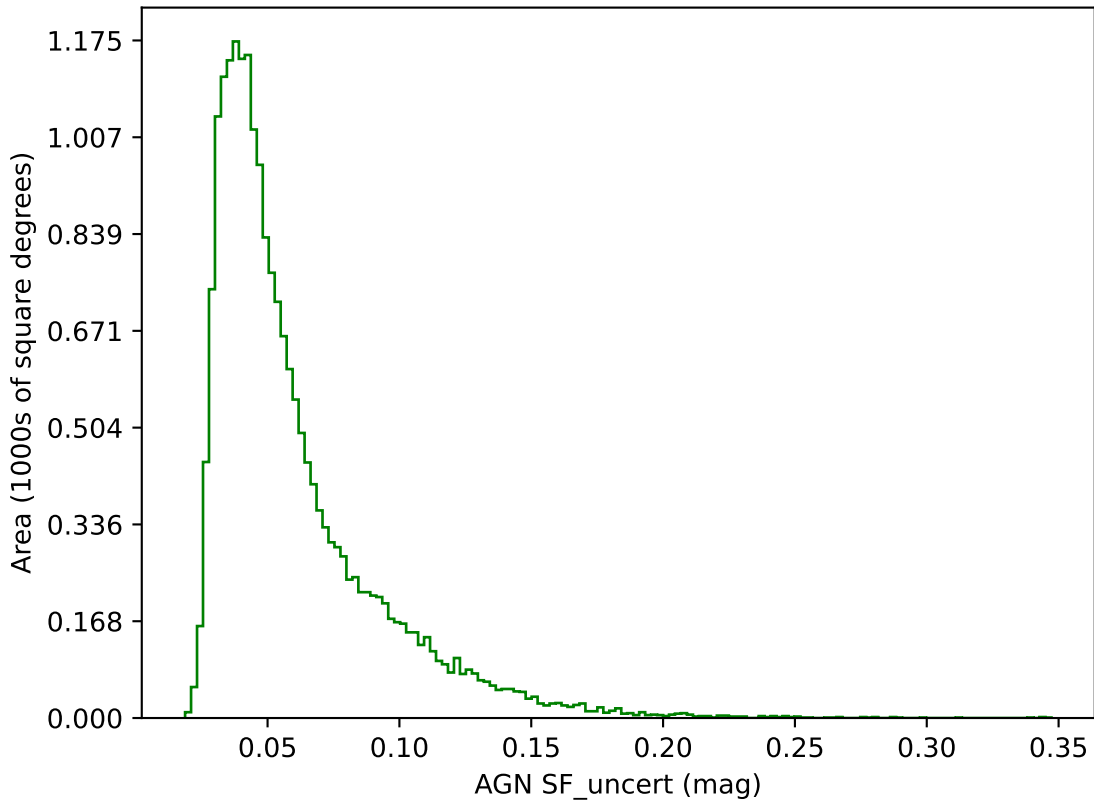
too_elab_r16_d3_giz_v3.4_10yrs g band: AGN SF_uncert
