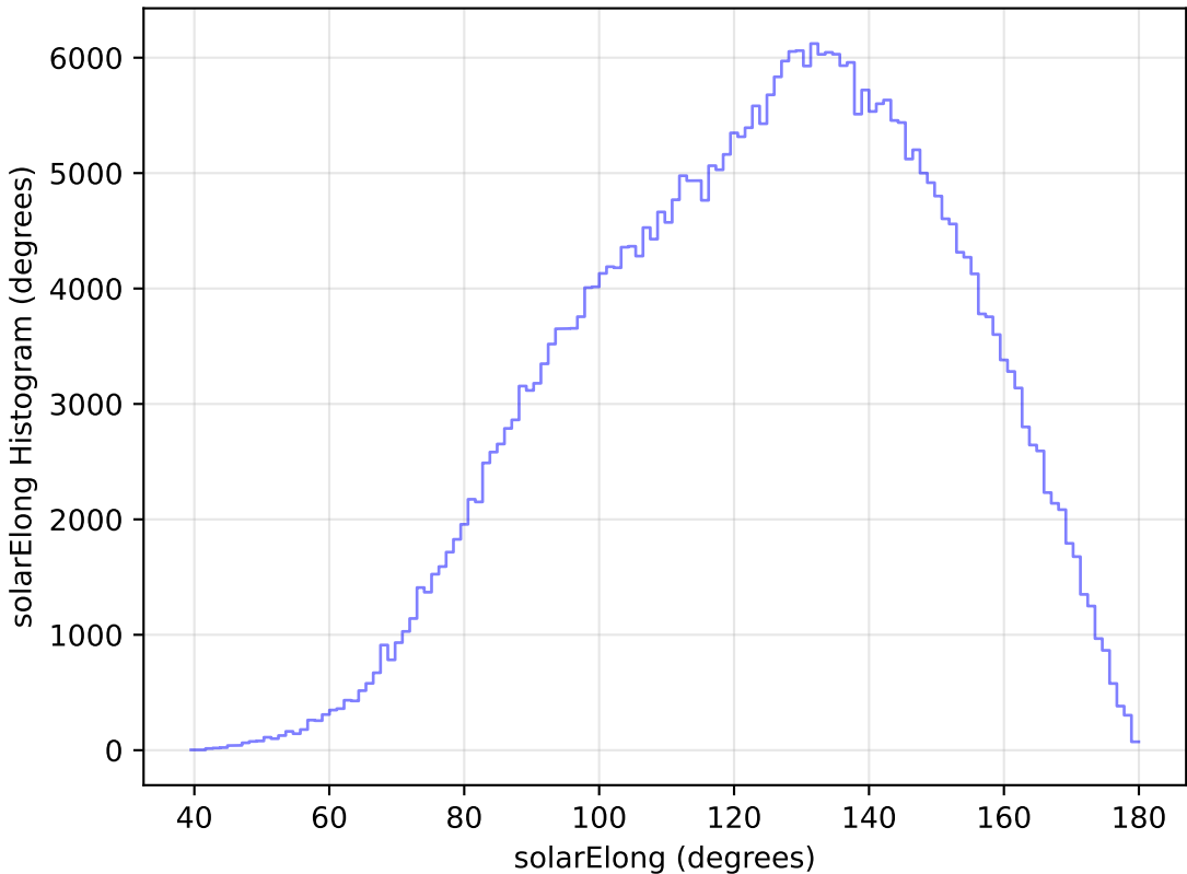
too_elab_r16_d3_giz_v3.4_10yrs WFD y band: solarElong Histogram
