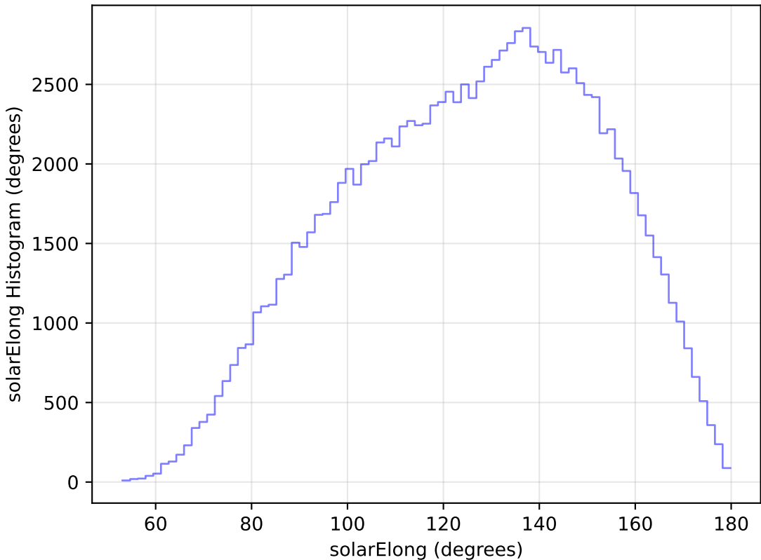
too_elab_r16_d3_giz_v3.4_10yrs WFD u band: solarElong Histogram
