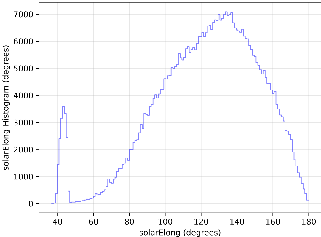
too_elab_r16_d3_giz_v3.4_10yrs WFD r band: solarElong Histogram
