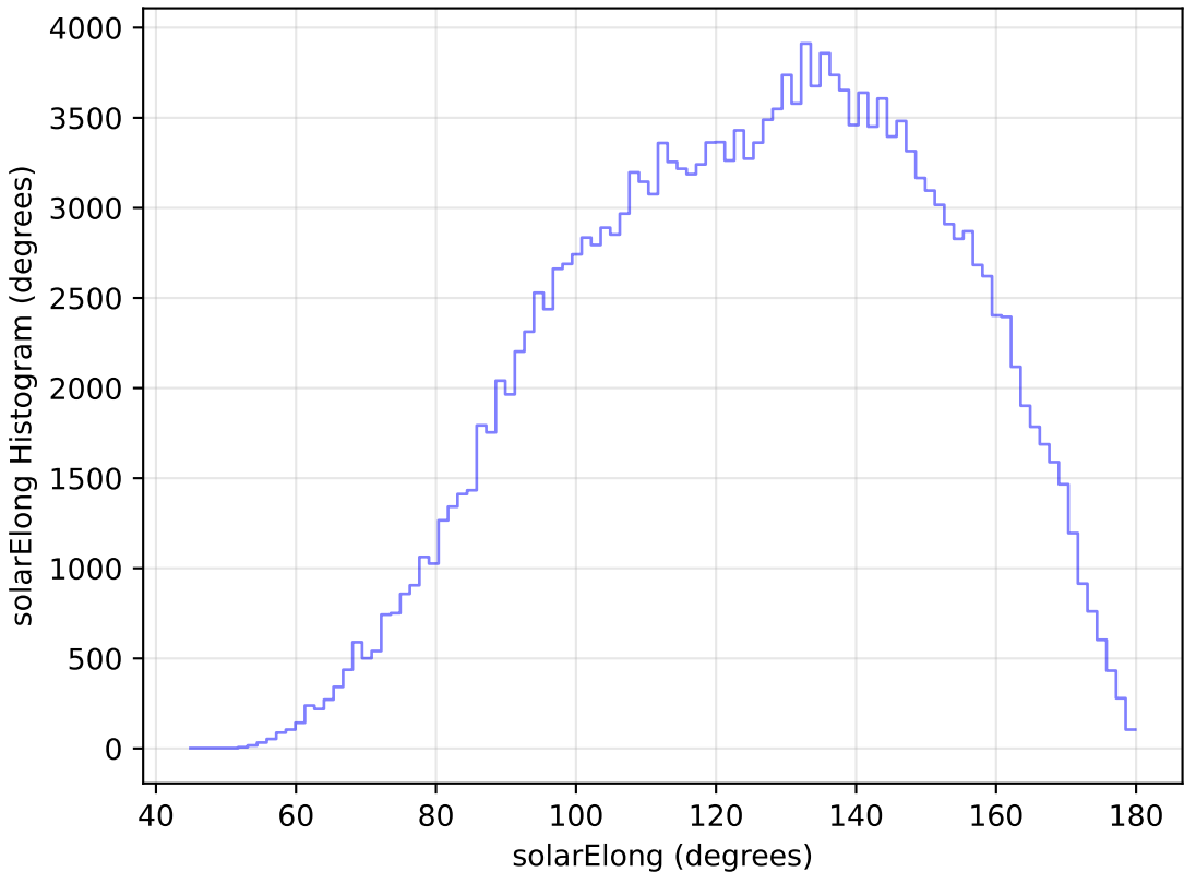
too_elab_r16_d3_giz_v3.4_10yrs WFD g band: solarElong Histogram
