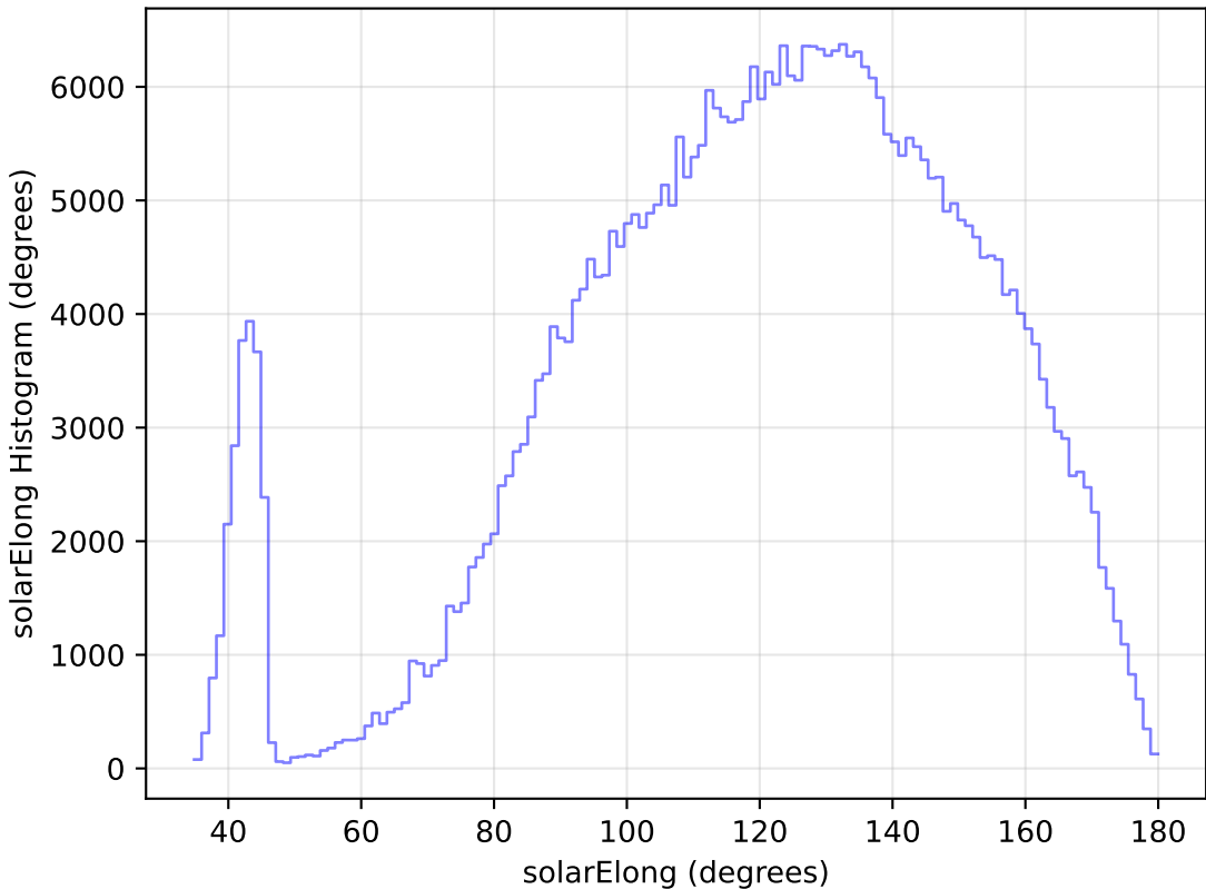
too_elab_r16_d3_giz_v3.4_10yrs All sky z band: solarElong Histogram
