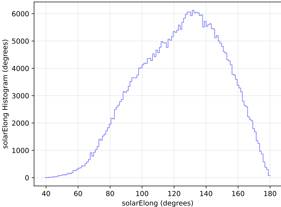
too_elab_r16_d3_giz_v3.4_10yrs All sky y band: solarElong Histogram
