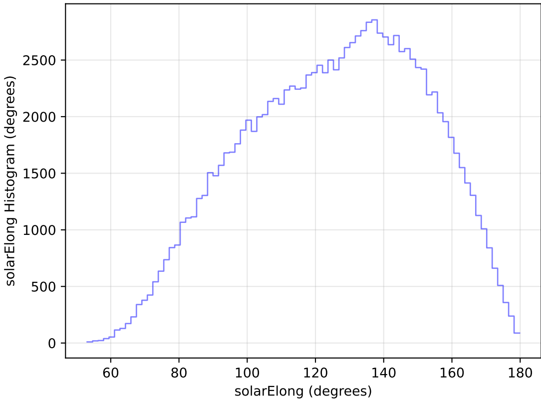
too_elab_r16_d3_giz_v3.4_10yrs All sky u band: solarElong Histogram
