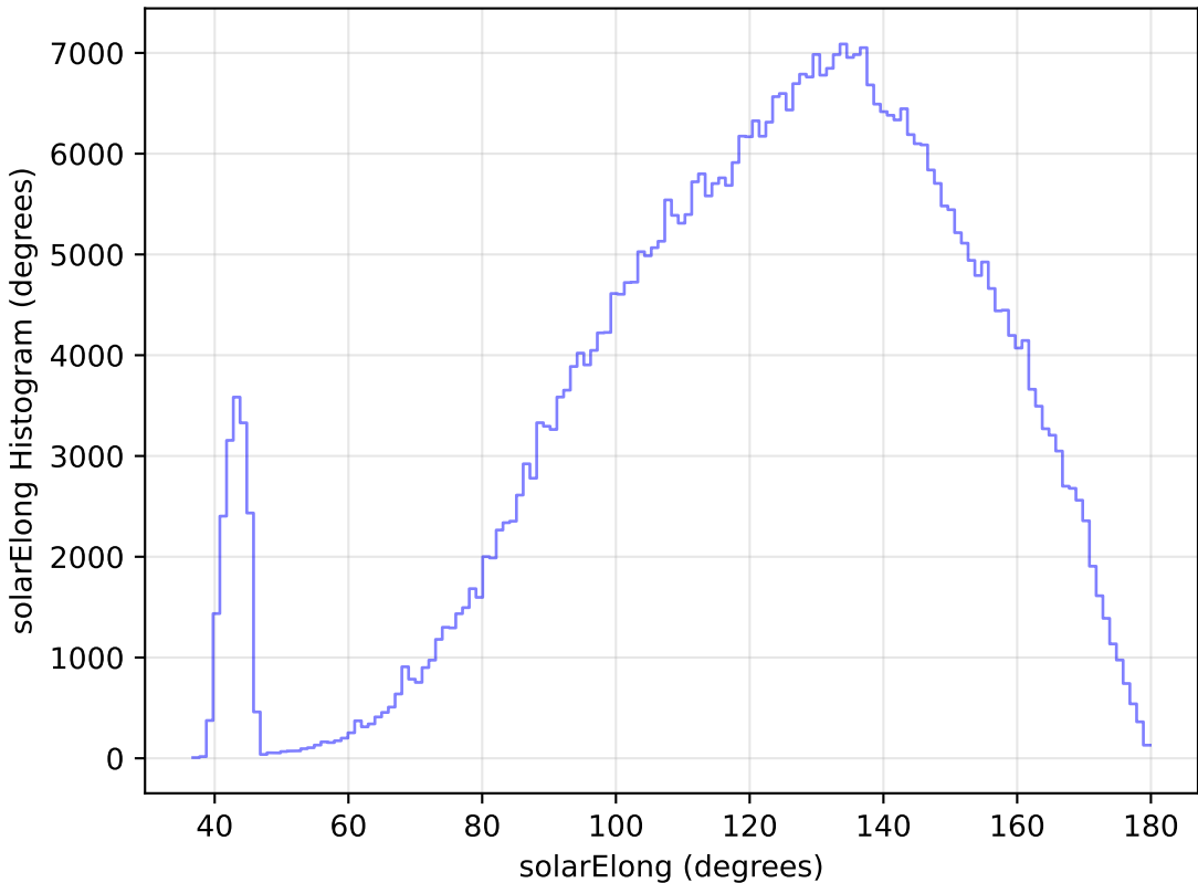
too_elab_r16_d3_giz_v3.4_10yrs All sky r band: solarElong Histogram
