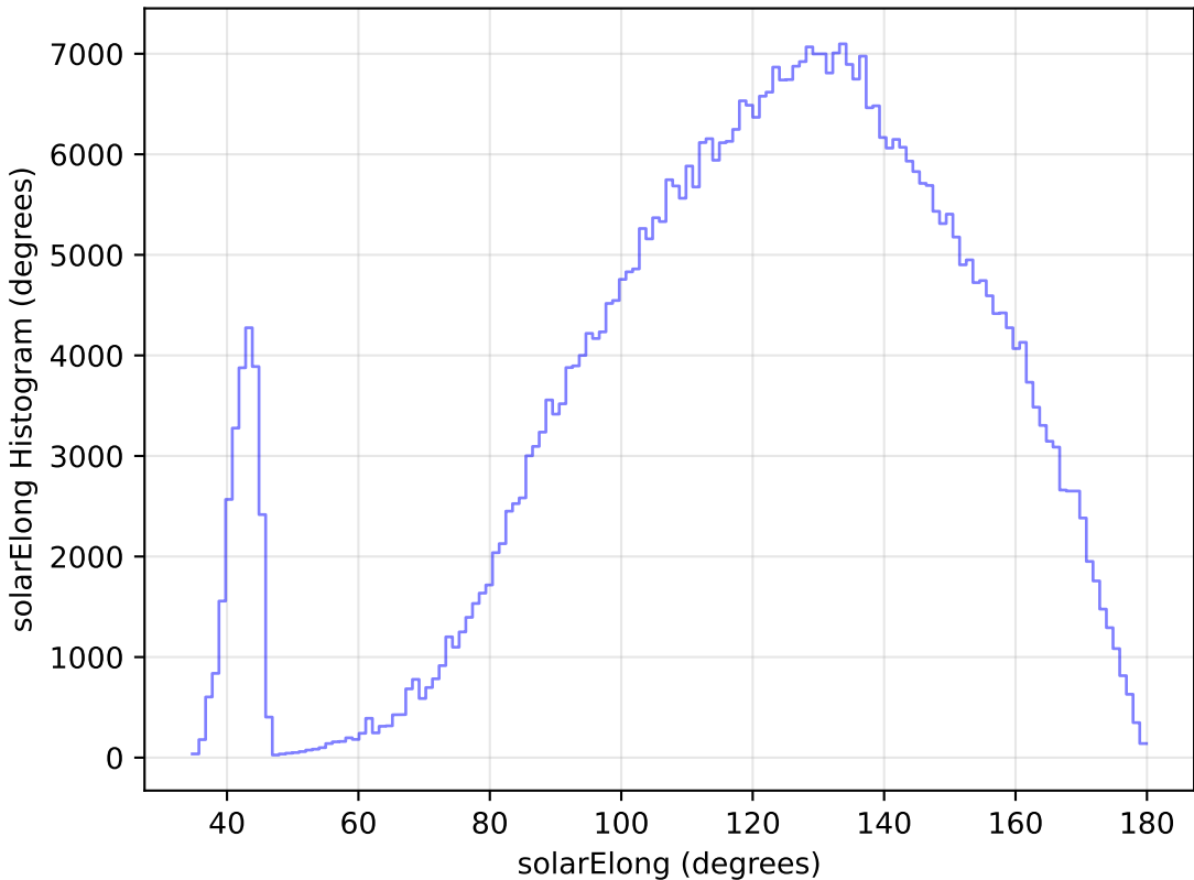
too_elab_r16_d3_giz_v3.4_10yrs All sky i band: solarElong Histogram
