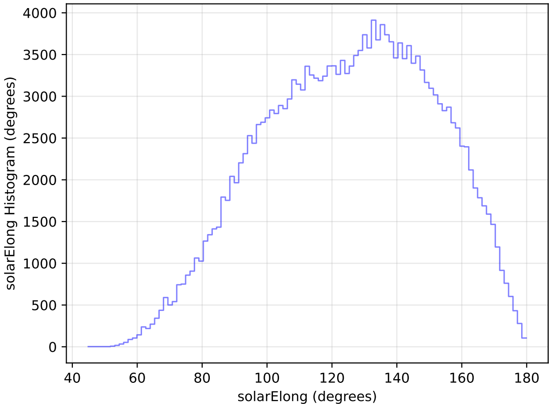
too_elab_r16_d3_giz_v3.4_10yrs All sky g band: solarElong Histogram
