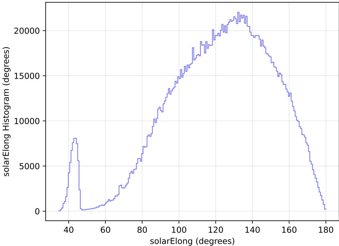
too_elab_r16_d3_giz_v3.4_10yrs All sky all bands: solarElong Histogram
