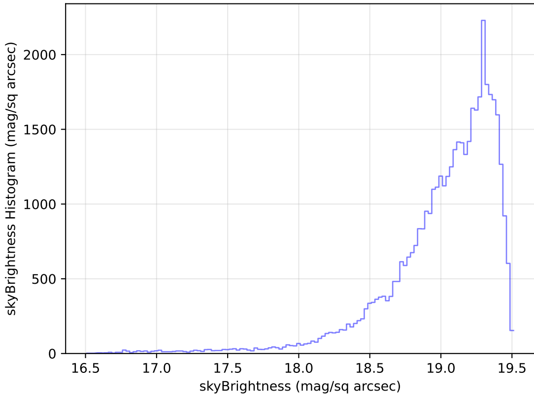
too_elab_r16_d3_giz_v3.4_10yrs Yr 1 z band: skyBrightness Histogram
