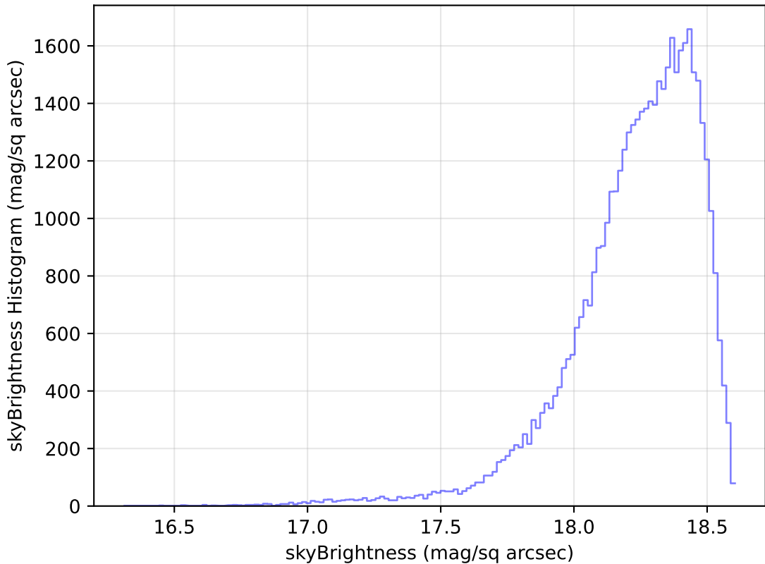
too_elab_r16_d3_giz_v3.4_10yrs Yr 1 y band: skyBrightness Histogram
