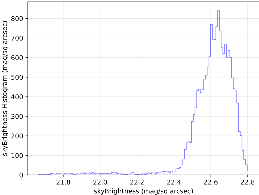
too_elab_r16_d3_giz_v3.4_10yrs Yr 1 u band: skyBrightness Histogram
