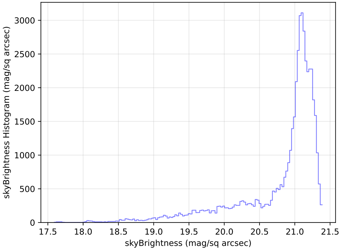
too_elab_r16_d3_giz_v3.4_10yrs Yr 1 r band: skyBrightness Histogram
