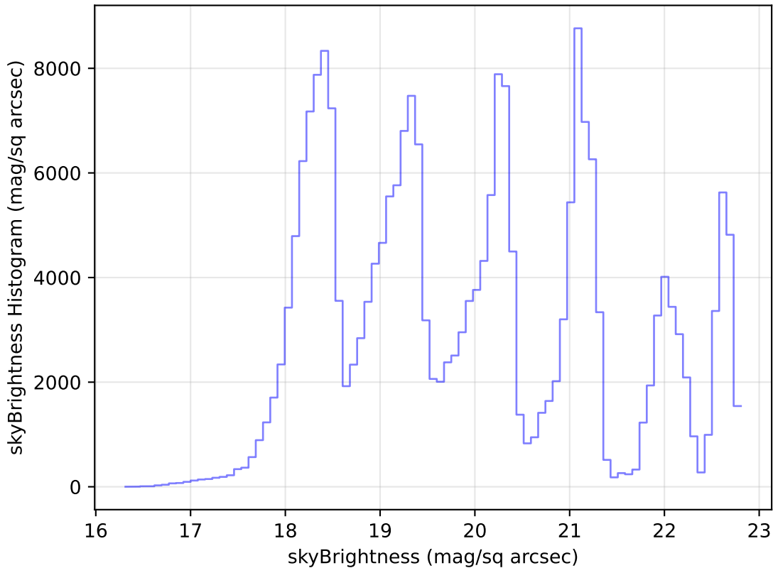
too_elab_r16_d3_giz_v3.4_10yrs Yr 1 all bands: skyBrightness Histogram
