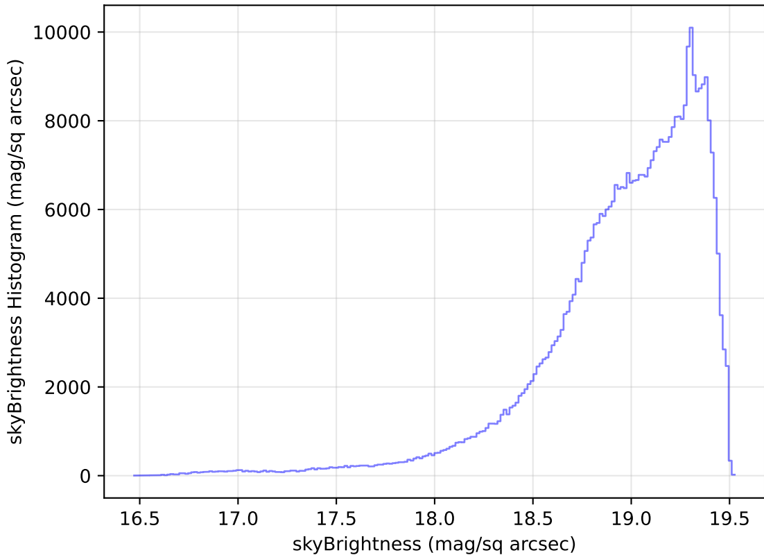
too_elab_r16_d3_giz_v3.4_10yrs WFD z band: skyBrightness Histogram
