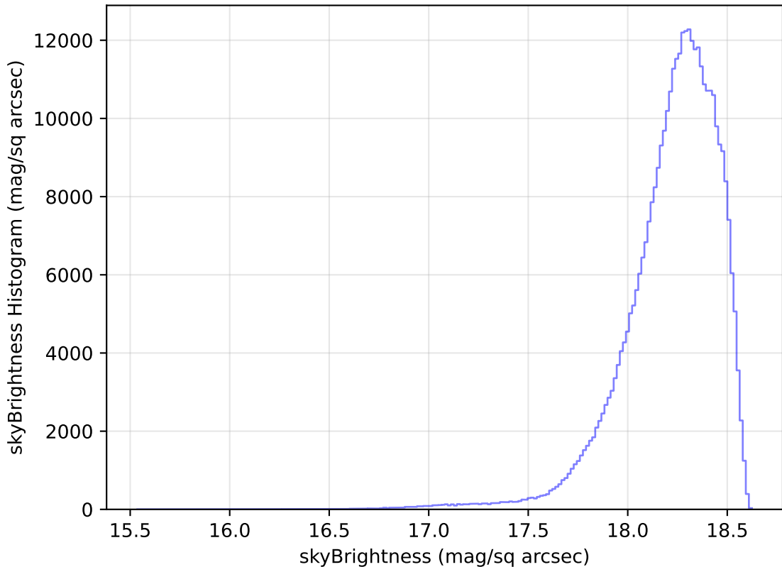
too_elab_r16_d3_giz_v3.4_10yrs WFD y band: skyBrightness Histogram
