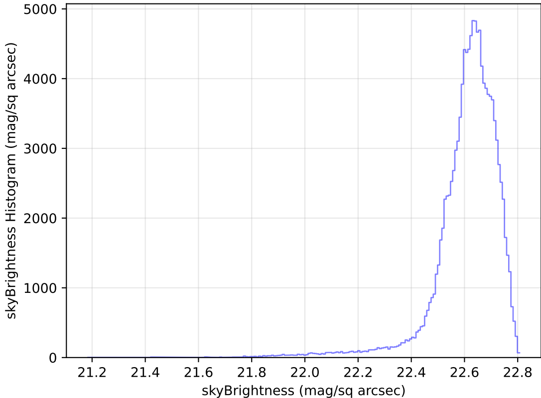
too_elab_r16_d3_giz_v3.4_10yrs WFD u band: skyBrightness Histogram
