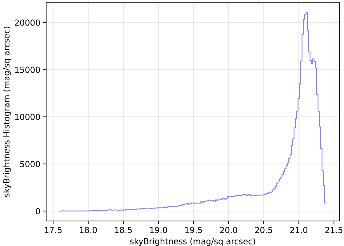
too_elab_r16_d3_giz_v3.4_10yrs WFD r band: skyBrightness Histogram
