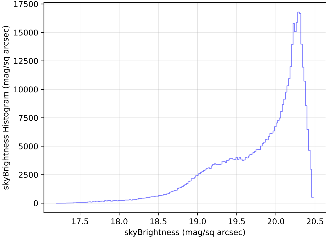
too_elab_r16_d3_giz_v3.4_10yrs WFD i band: skyBrightness Histogram
