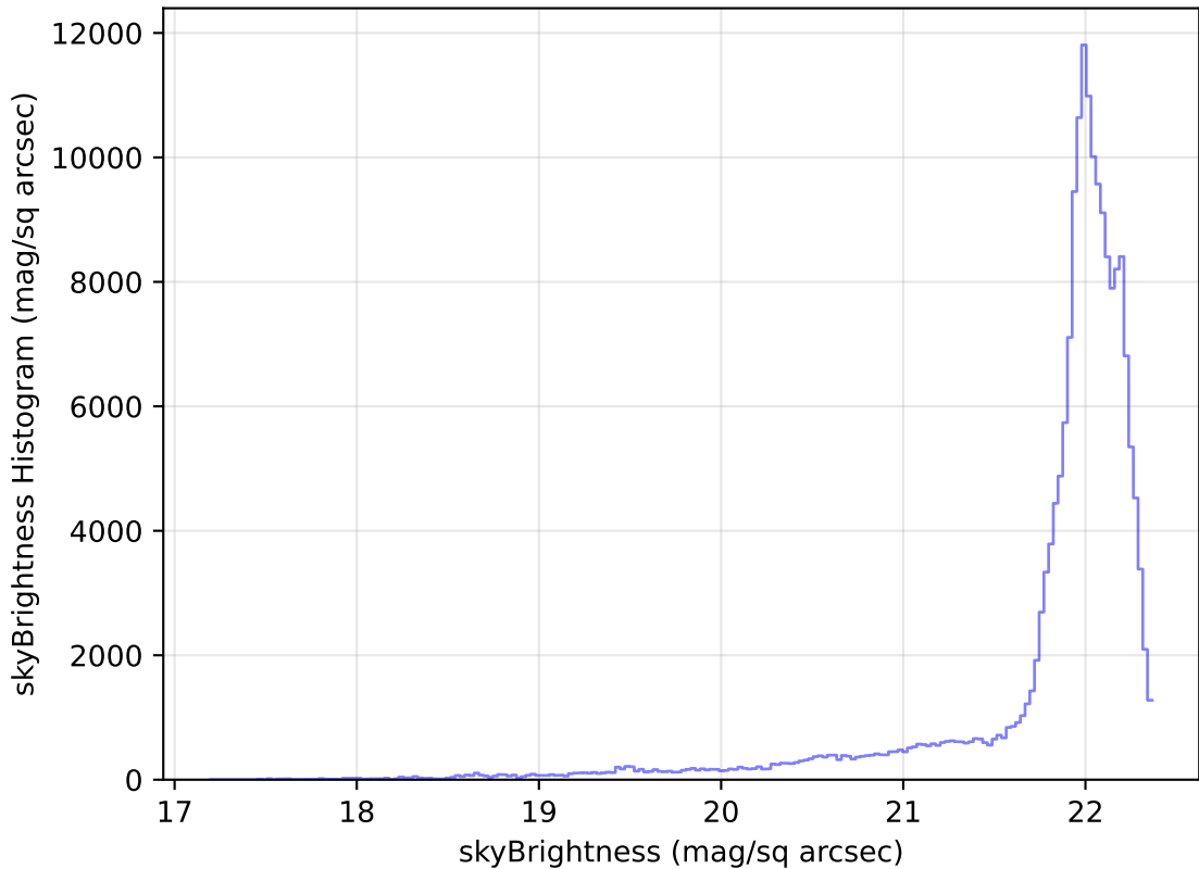
too_elab_r16_d3_giz_v3.4_10yrs WFD g band: skyBrightness Histogram
