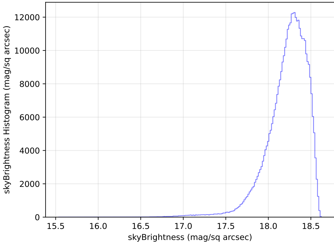
too_elab_r16_d3_giz_v3.4_10yrs All sky y band: skyBrightness Histogram
