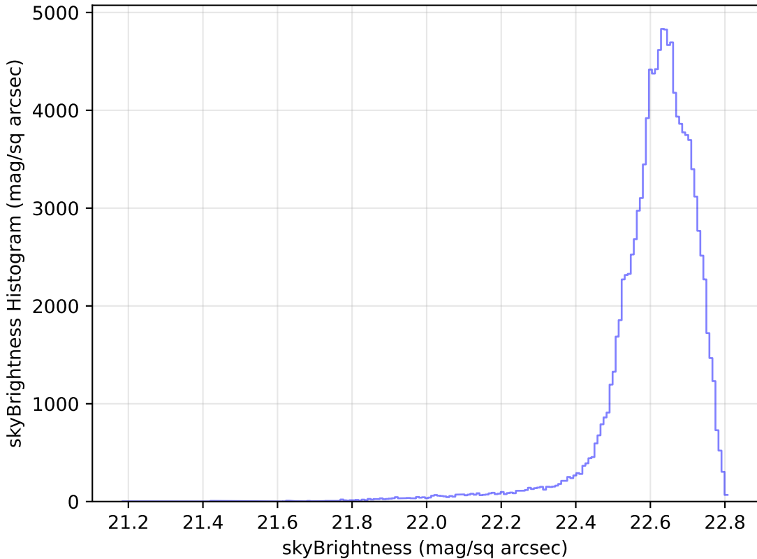
too_elab_r16_d3_giz_v3.4_10yrs All sky u band: skyBrightness Histogram
